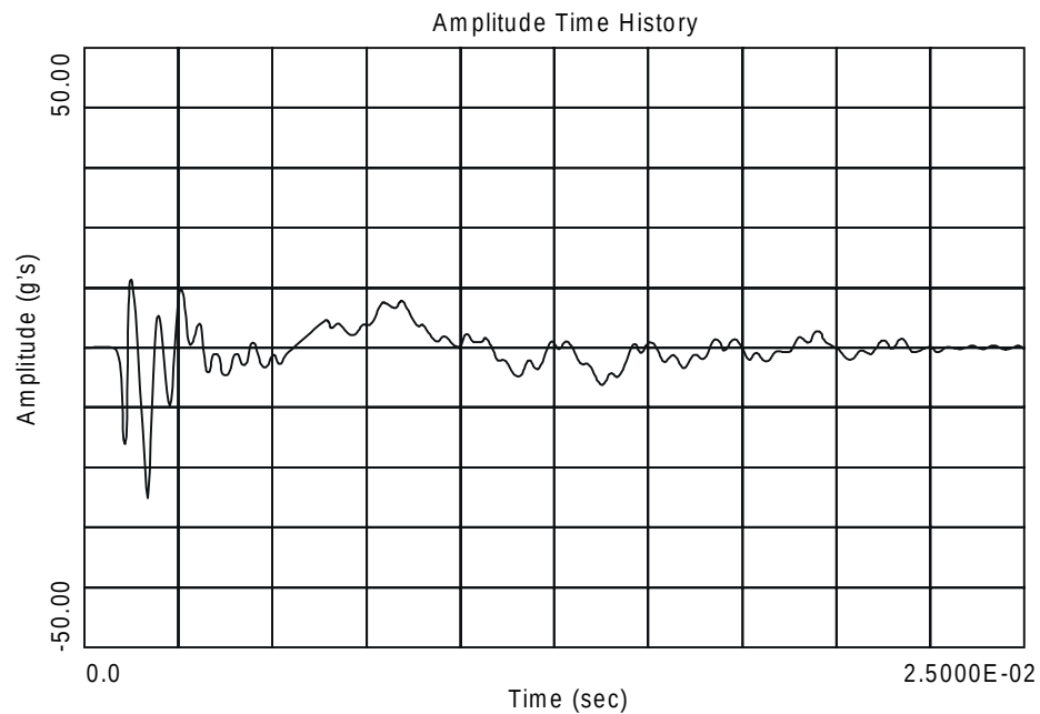
FIGURE 519.5C-3. SRS gunfire pulse generated using a digital controller.
